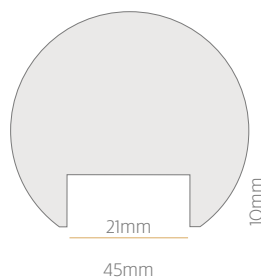
45mm - Rebate TL 806
